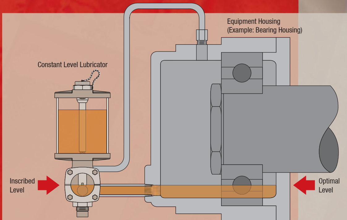
Fig. 1 - Installation Height
